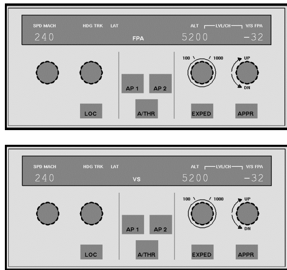
Figure 2. Flight Control Unit (FCU), Set for Descents of 3.2° and 3200 fpm
