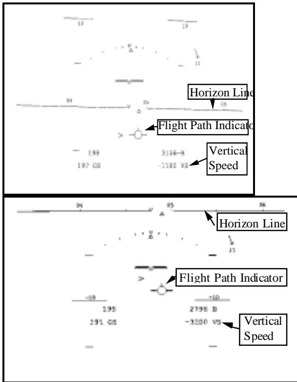
Figure 1. Heads Up Display in 3.2° and 3200 fpm Descent Modes
