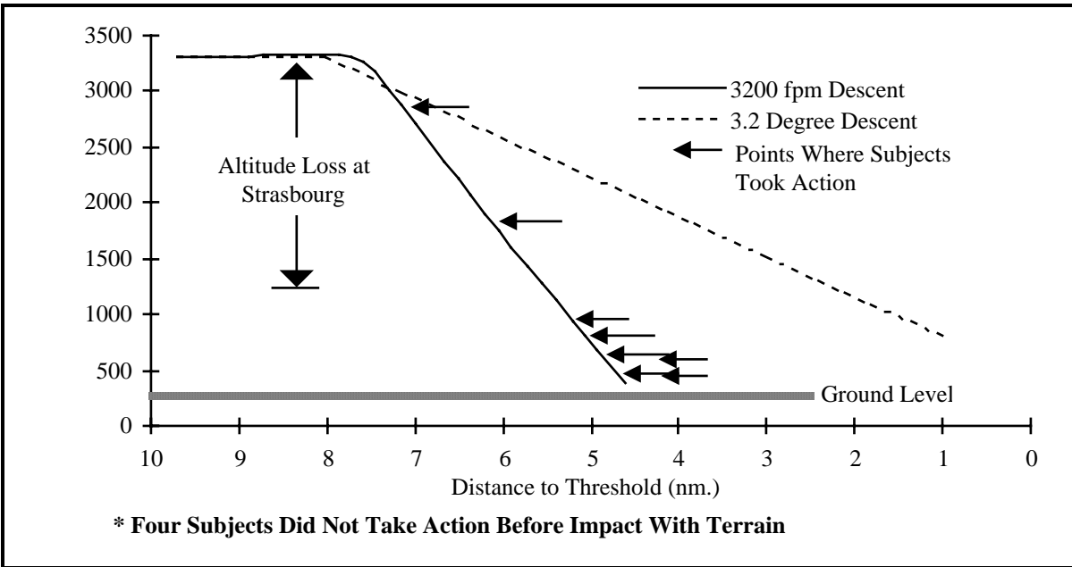
Fig. 3. Altitudes At Which Pilots Took Action
