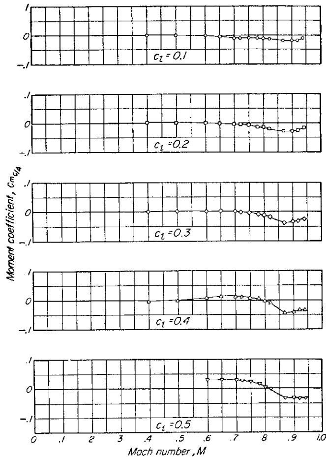
FIG. 181. Effect of compressibility on the pitching moment of the NACA 0006-34 airfoil.
