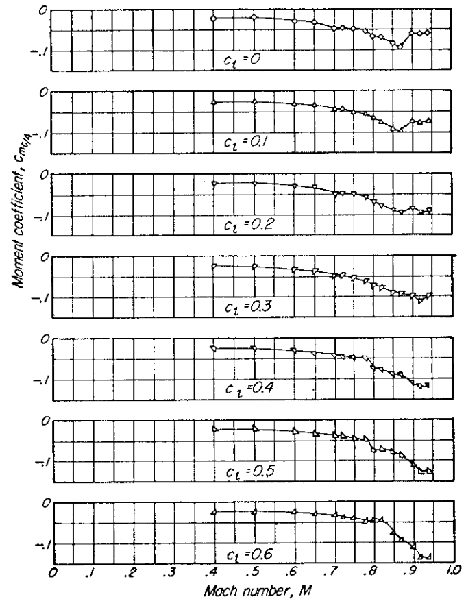
FIG. 182. Effect of compressibility on the pitching moment of the NACA 2306 airfoil.
