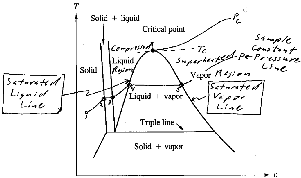
Figure 2.6 The T-v projection of an equilibrium diagram for a substance that contracts upon freezing.
